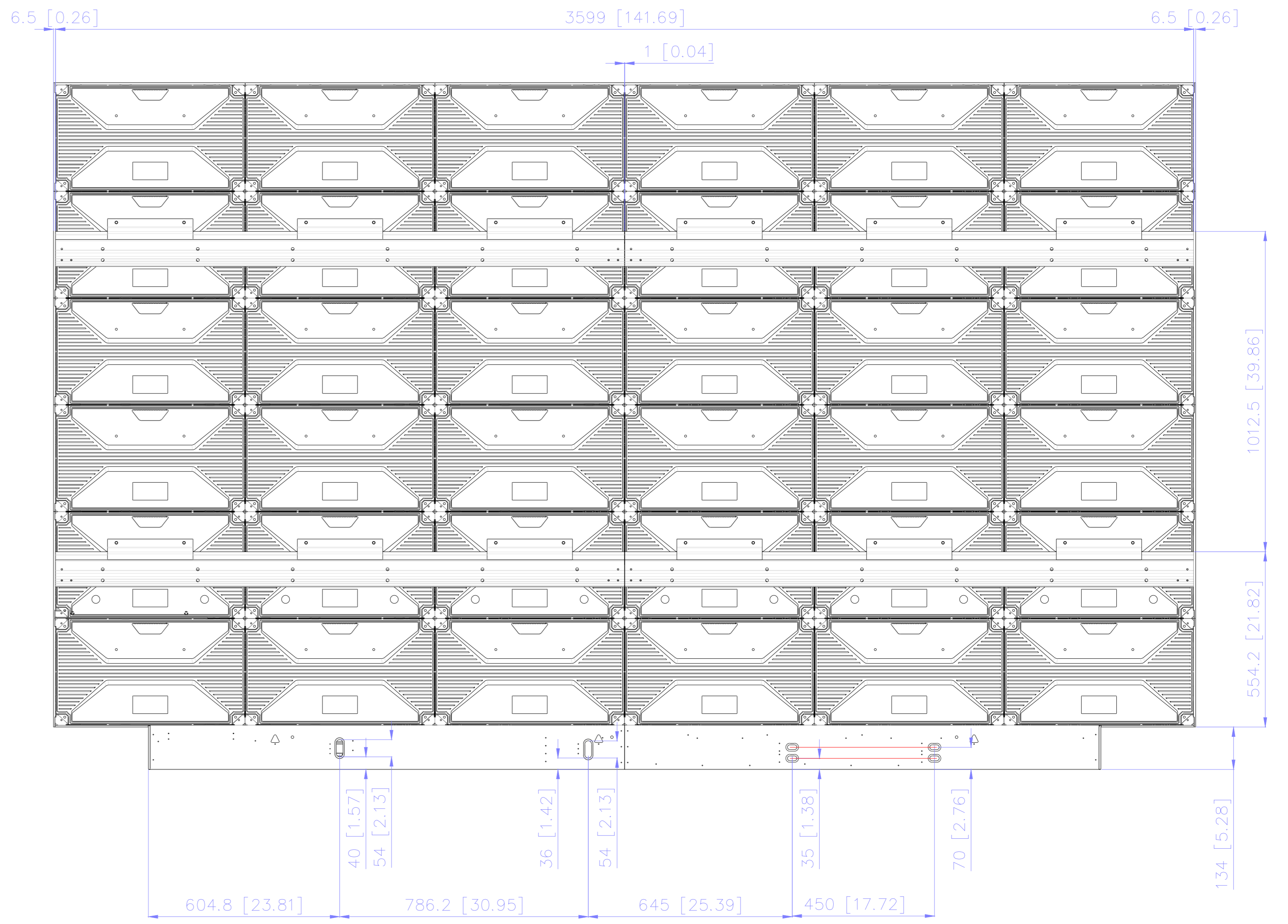
Rear View
