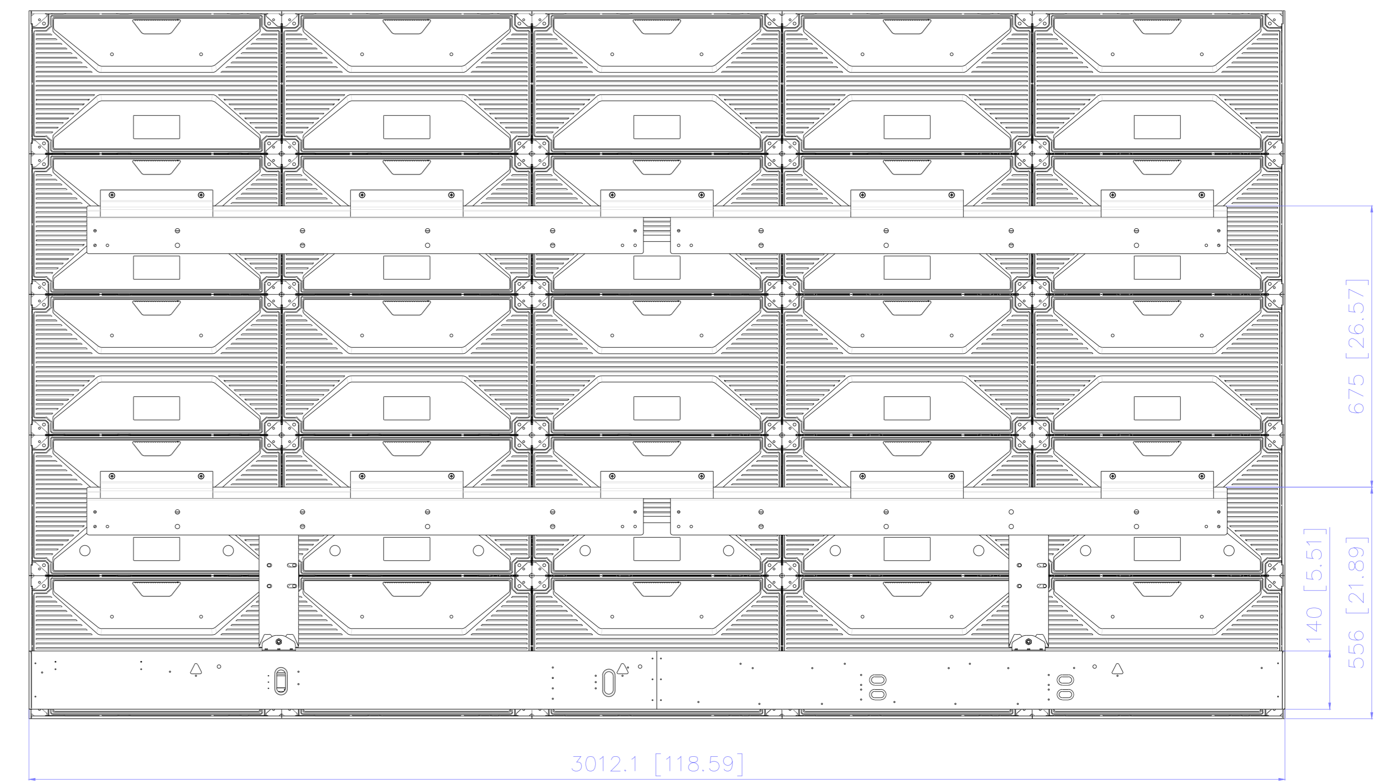
Rear View
